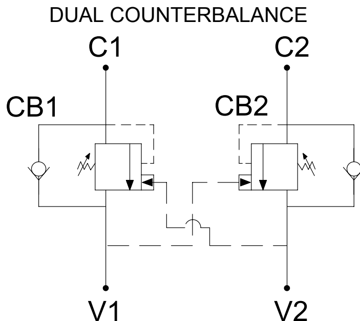
CIRCUIT LA
